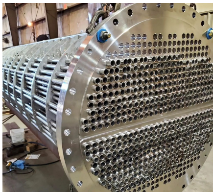
HEAT EXCHANGER RETUBING/FABRICATION
